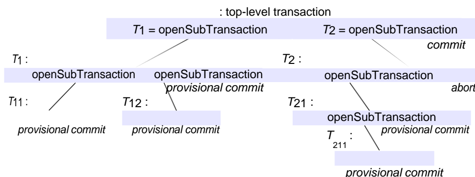
Figure 16.13 Nested transactions
